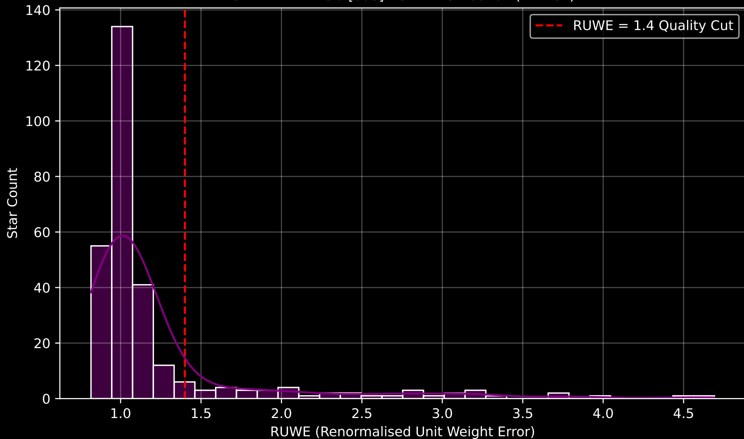
GALAH DR4 Field [608] RUWE Distribution (n= 287)
