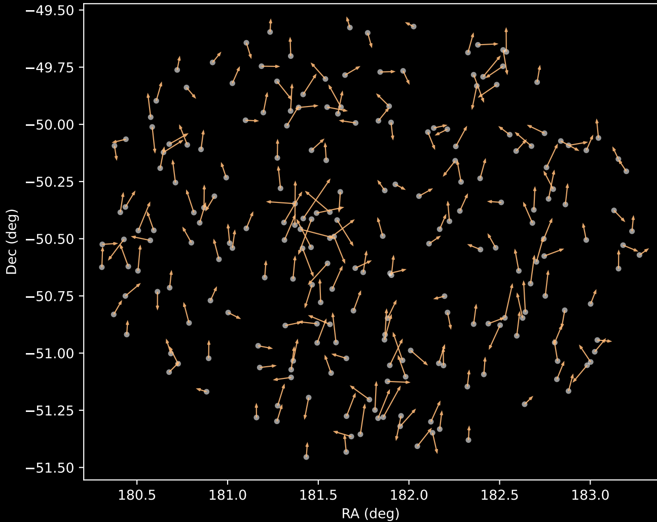
GALAH DR4 Cluster 3 Proper Motion Vectors (n=223)
