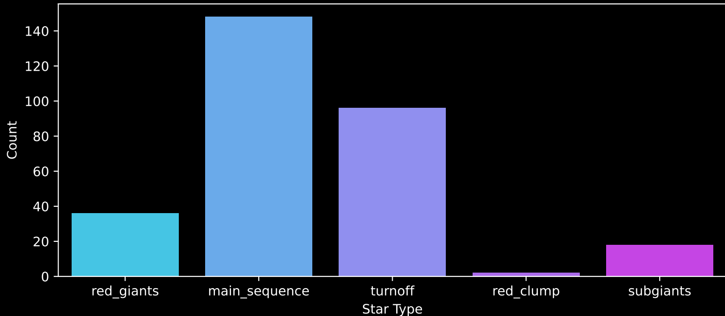
GALAH DR4 Field: [608] Count plot of Star Type
