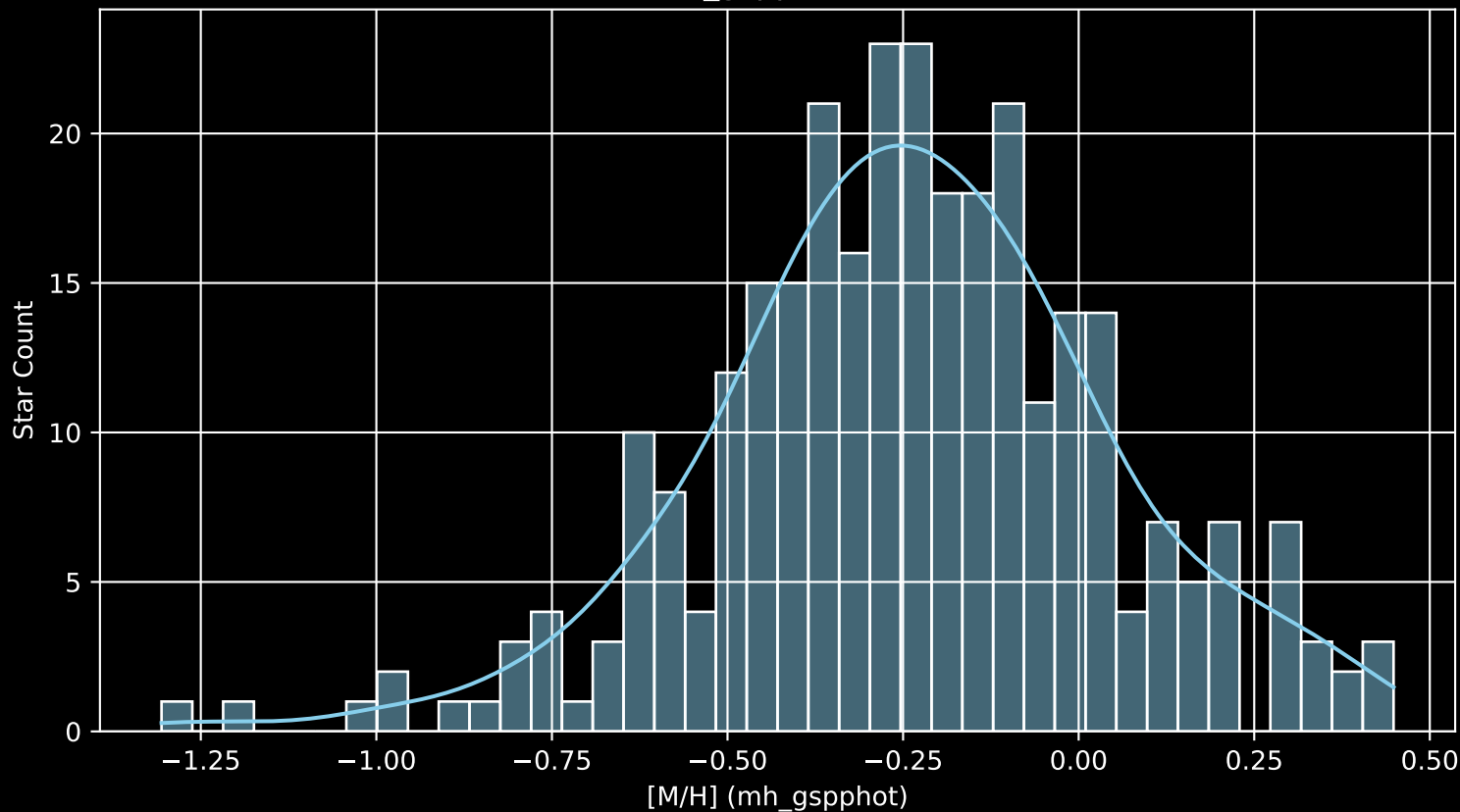
GALAH DR4 Field: [608] [M/H] (mh_gspphot) (n= 299)
