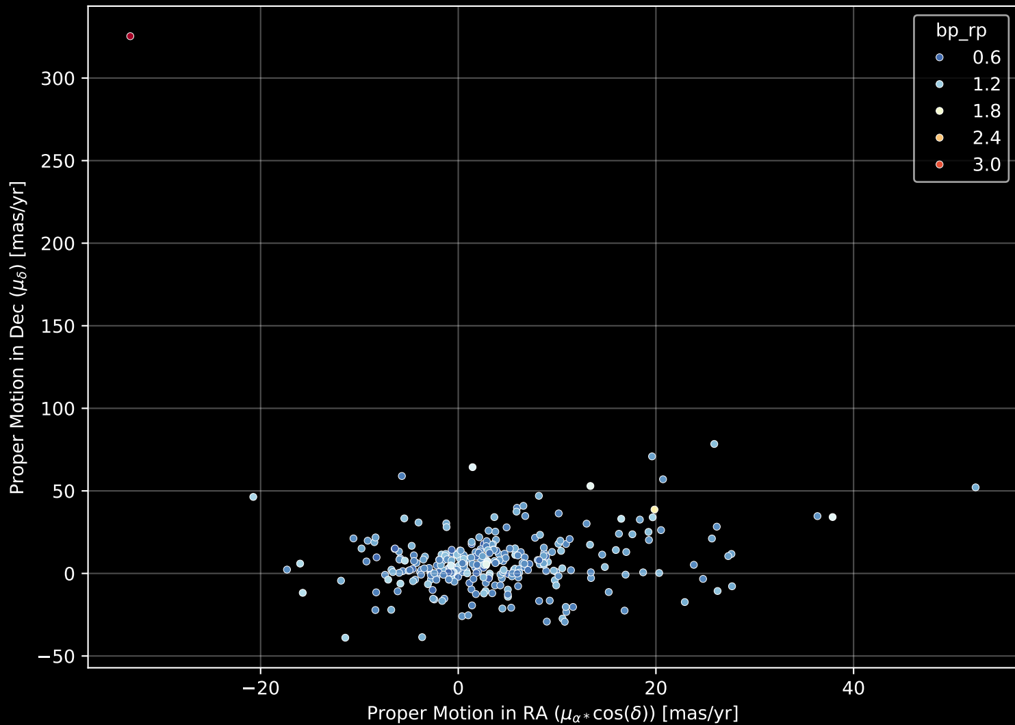
GALAH DR4 Field: [608] Proper Motion Diagram (n= 300)
